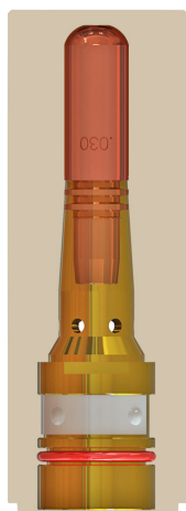
64-2387 7/8" Bore 1/4" Recess Brass 1.062" O.D. Straight Bore
